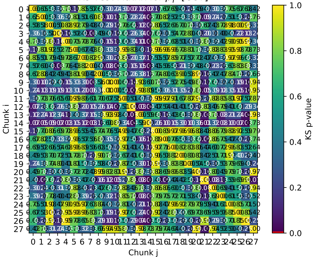
KS Test Matrix for p_T^{j1} [GeV]
