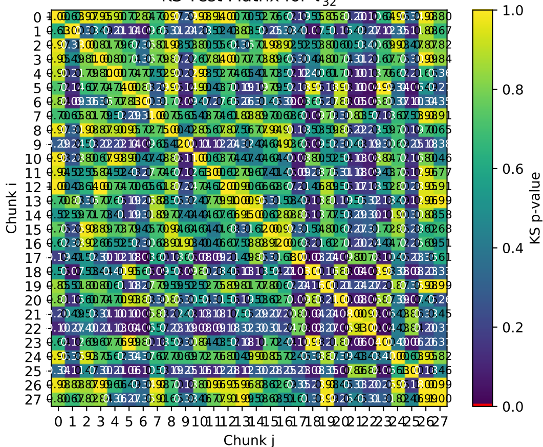
KS Test Matrix for \tau_{32}^{/1}
