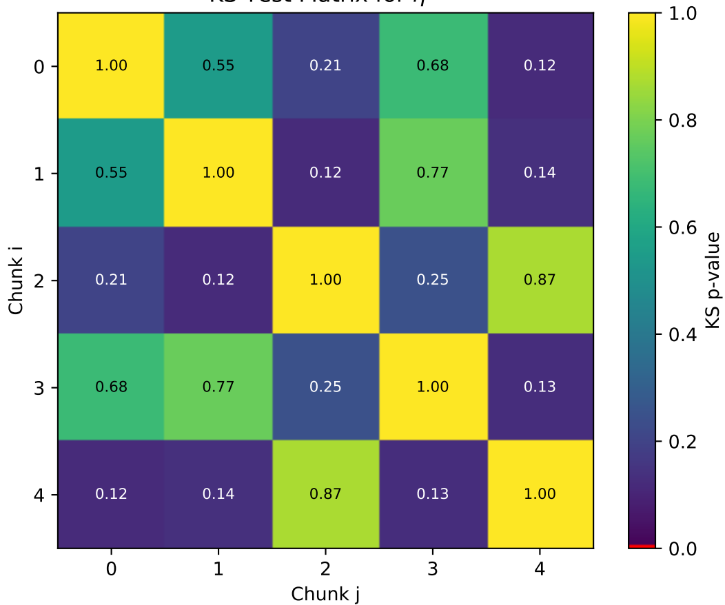
KS Test Matrix for \eta^{j^2}
