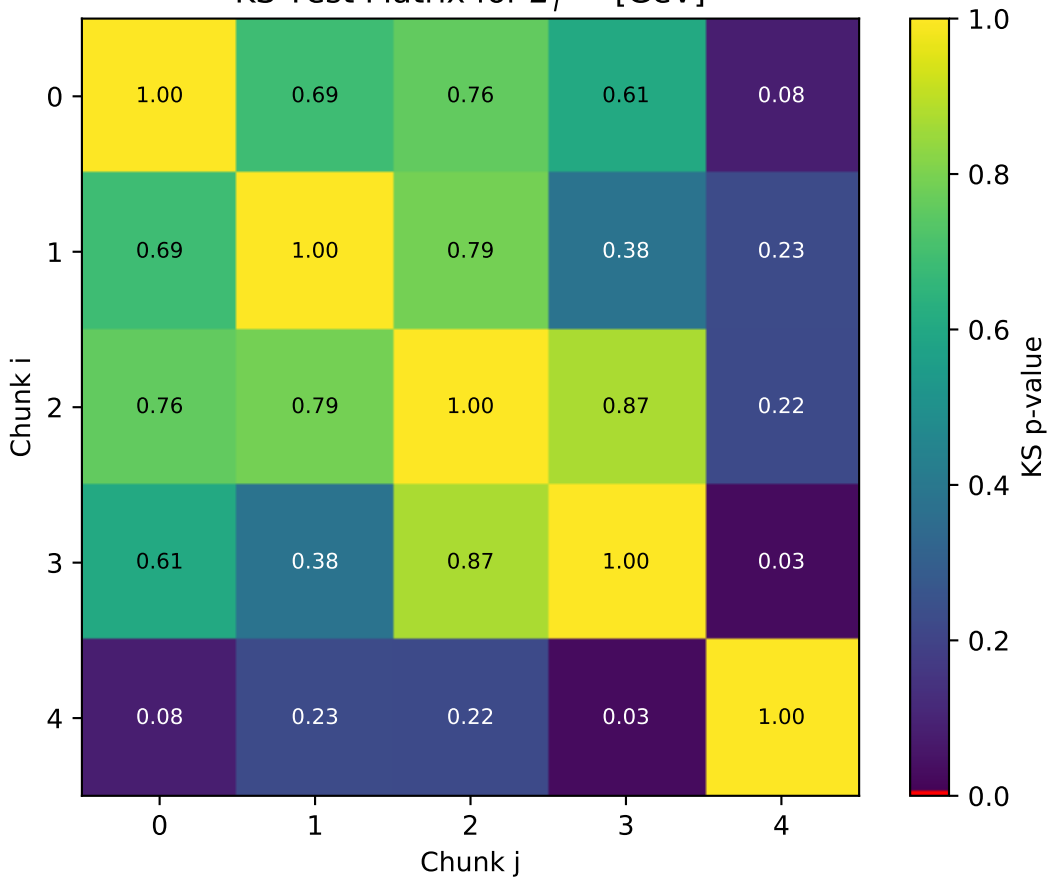
KS Test Matrix for E_T^{miss} [GeV]
