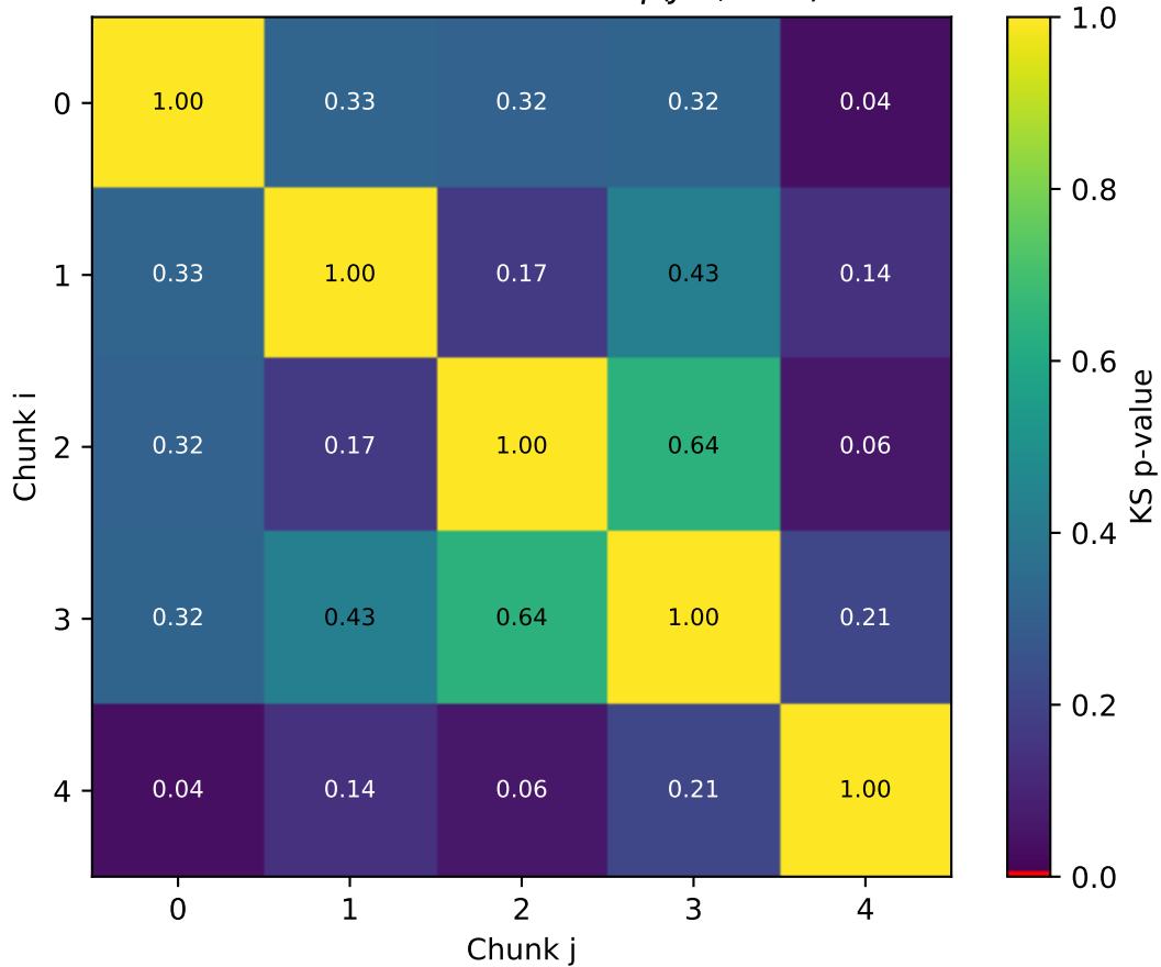
KS Test Matrix for \min\Delta\phi(\text{jet}, \text{MET})
