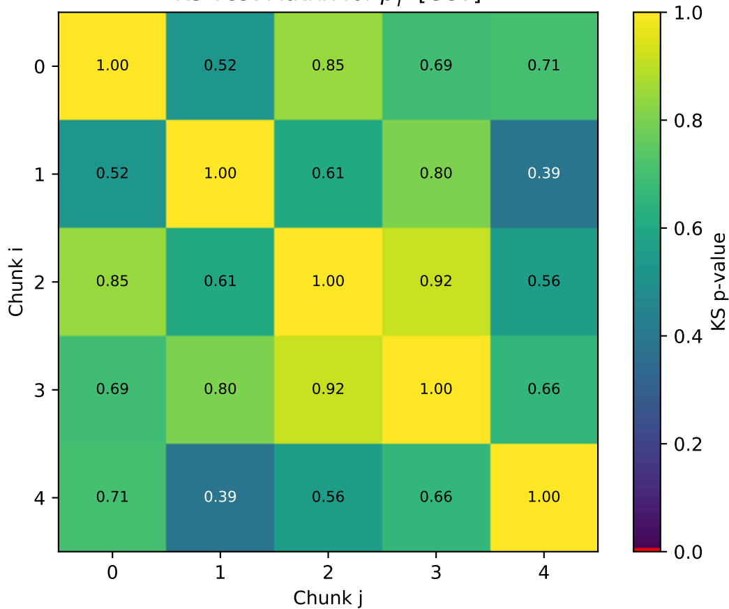
KS Test Matrix for p_T^{j1} [GeV]
