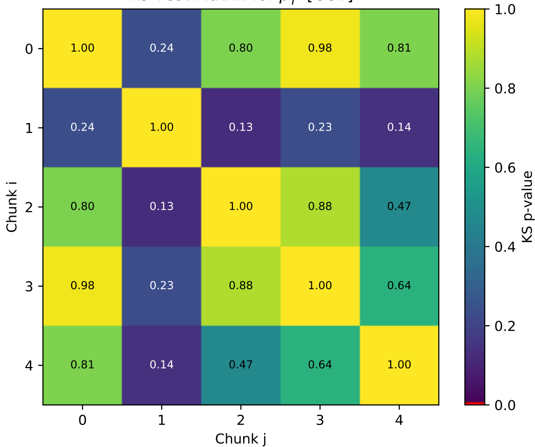
KS Test Matrix for p_T^{j2} [GeV]
