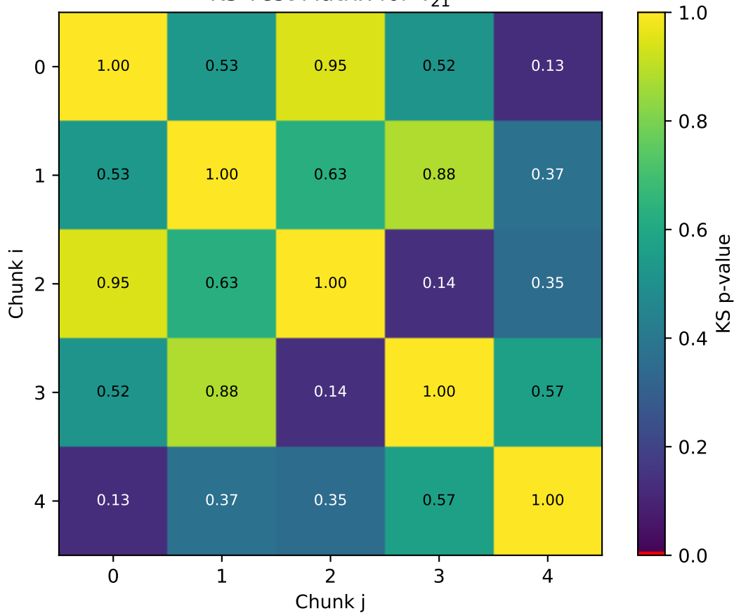
KS Test Matrix for \tau_{21}^{j1}
