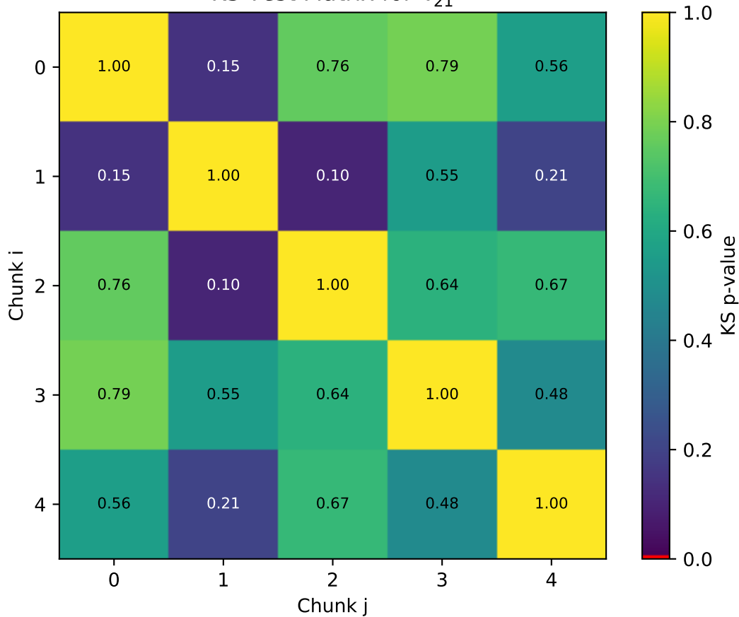
KS Test Matrix for \tau_{21}^{j2}
