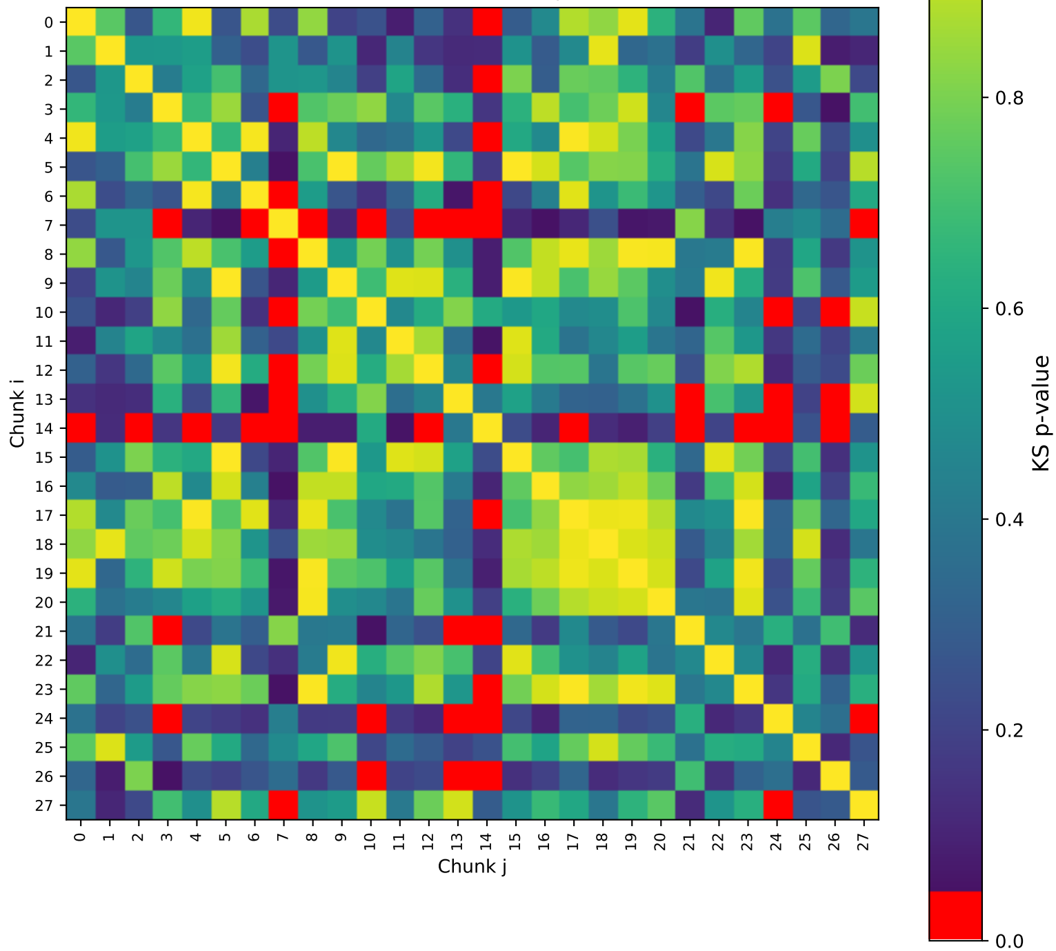
KS Test Matrix for H_T [GeV]
