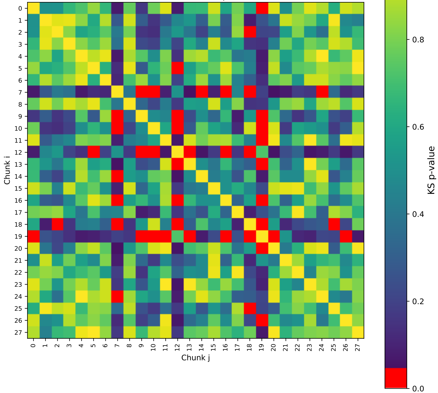
KS Test Matrix for E_T^{miss} [GeV]
