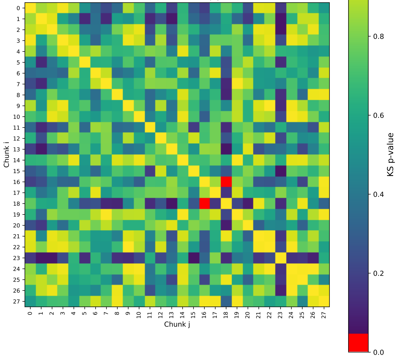
KS Test Matrix for \min\Delta\phi(\text{jet}, \text{MET})
