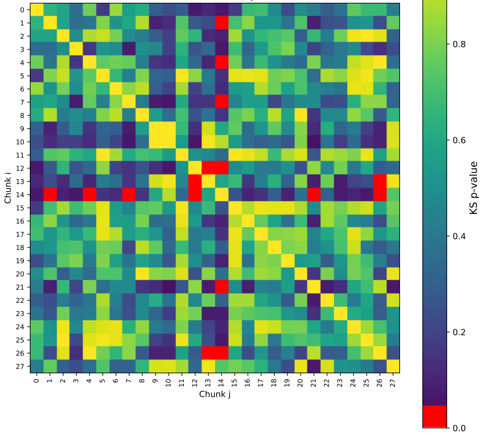
KS Test Matrix for p_T^{j1} [GeV]
