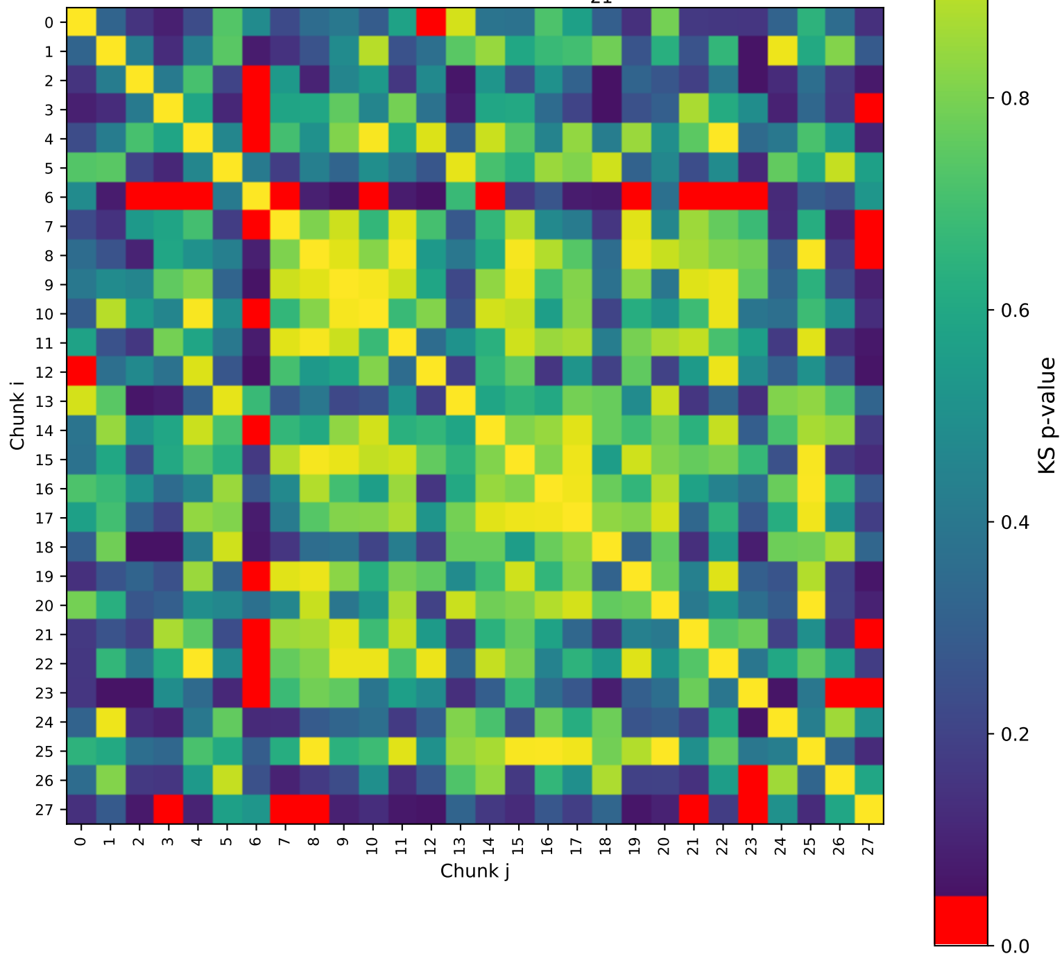
KS Test Matrix for \tau_{21}^{j1}
