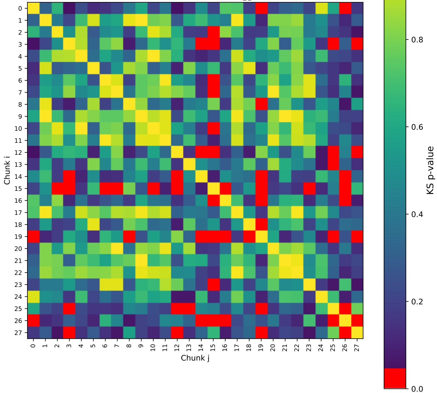
KS Test Matrix for \tau_{21}^{j2}
