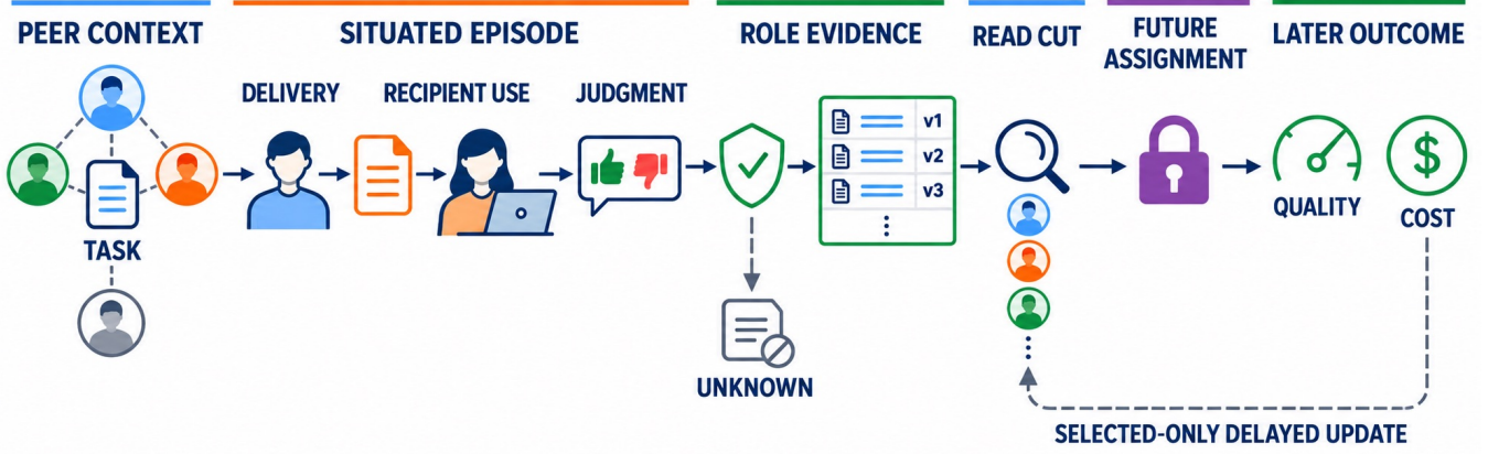
Figure 1: The earning-roles protocol. Orange marks situated observation; green marks producer-attributable evidence, while the UNKNOWN branch remains audit-only; blue marks the sealed assignment and scored outcome. Gray dashed feedback is delayed and selected-only, entering a future state and next read cut without changing historical evidence or a sealed assignment. Peer-context links are descriptive, not causal.
