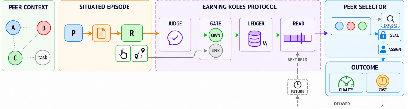
Figure 1: The earning-roles protocol. Orange marks situated observation; green marks producer-attributable evidence, while the UNKNOWN branch remains audit-only; blue marks the sealed assignment and scored outcome. Gray dashed feedback is delayed and selected-only, entering a future state and next read cut without changing historical evidence or a sealed assignment. Peer-context links are descriptive, not causal.
