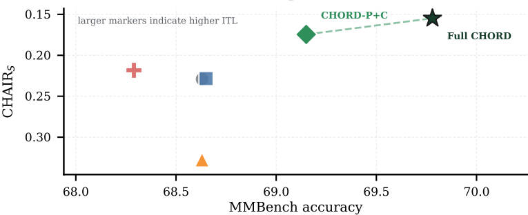
(c) LLaVA-v1.5-7B trade-off map
