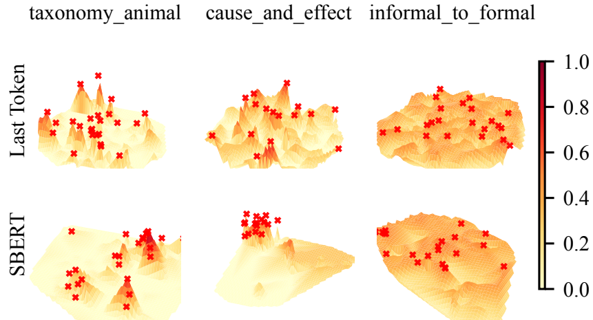
Figure[R] 1: The t-SNE visualized function surfaces using the (Vicuna-13B) last token or SBERT embedding, and the local optima (marked in "x") identified in the original space.
