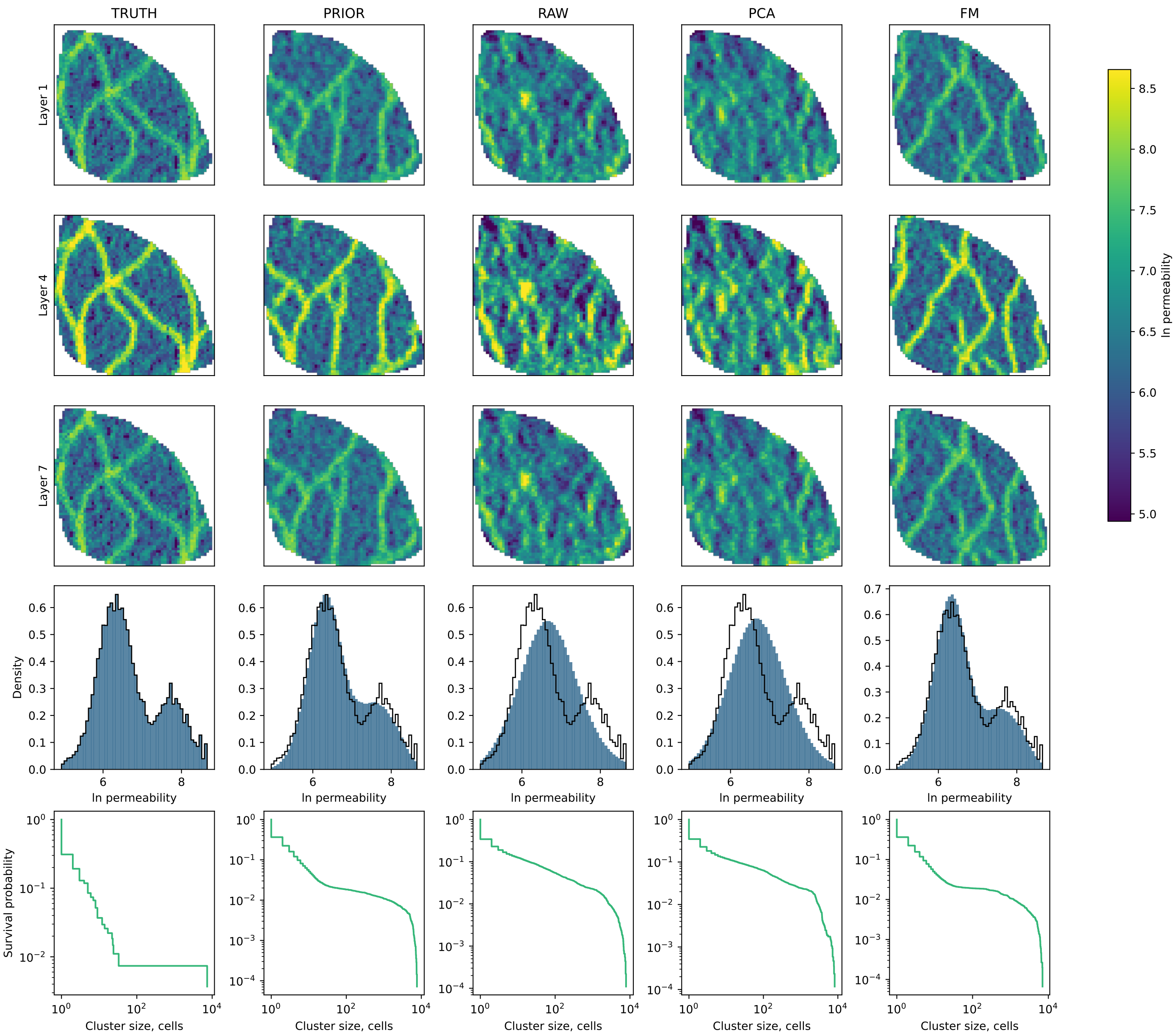
Egg held-out inversion: selected fields and ensemble geology
