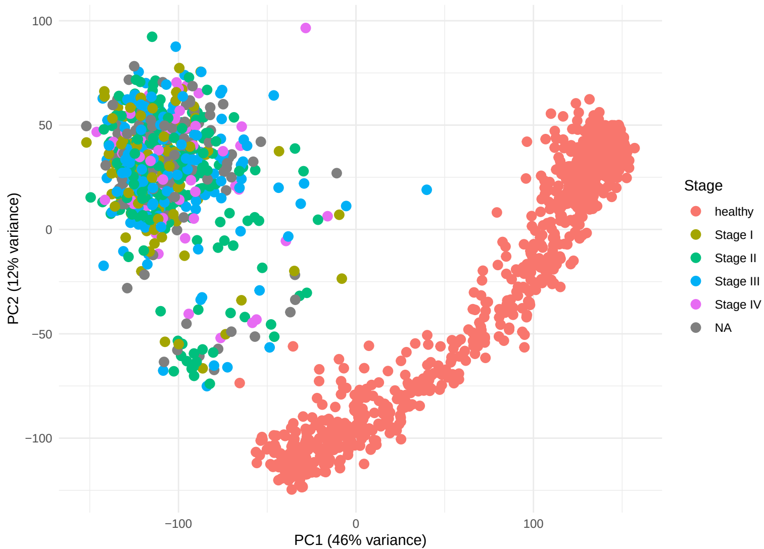
PCA gene expression | Colored by stage
