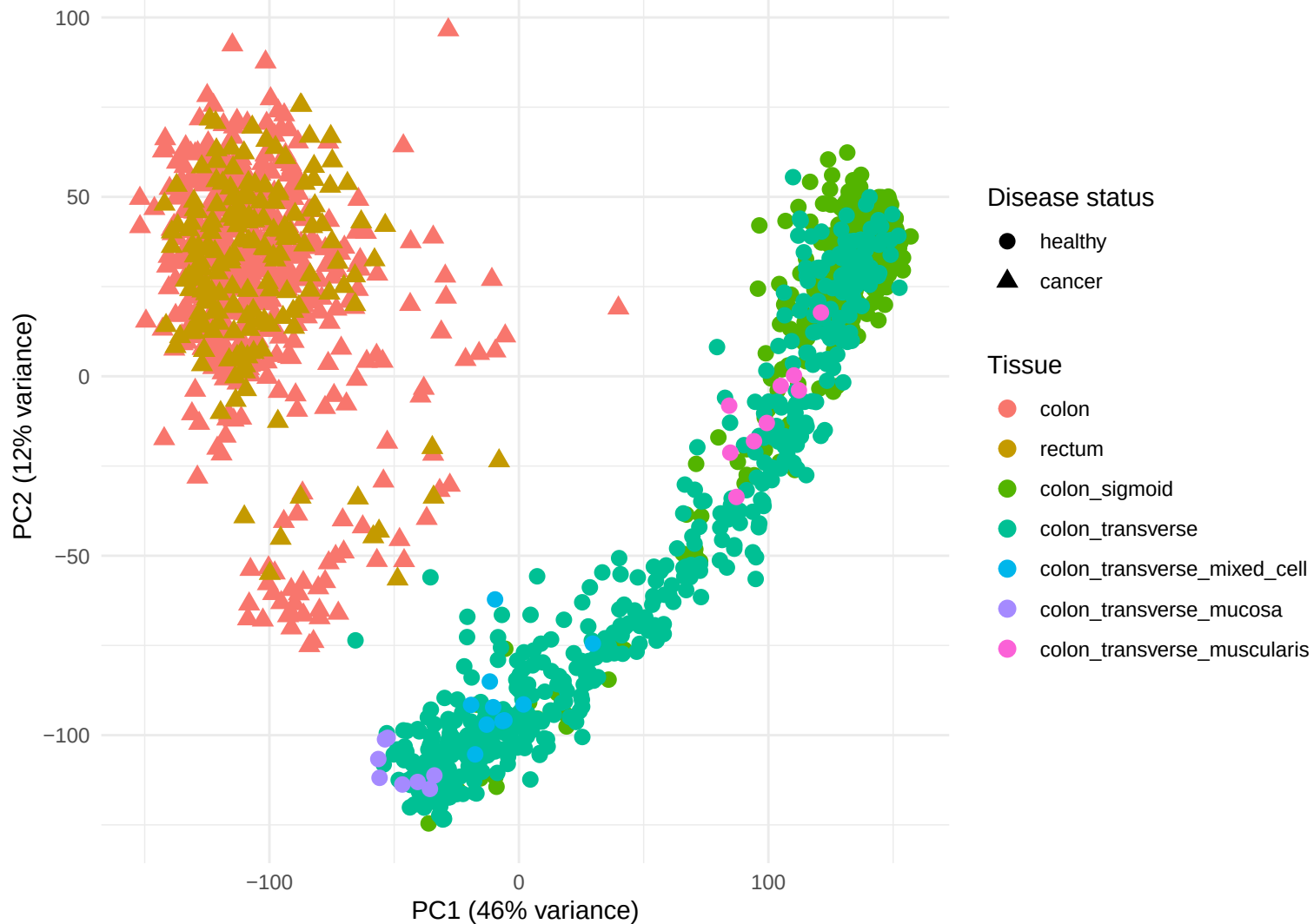
PCA gene expression | Colored by tissue | Shape by disease status
