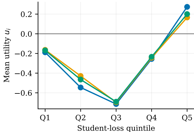
T_{a00} gold-token utility
