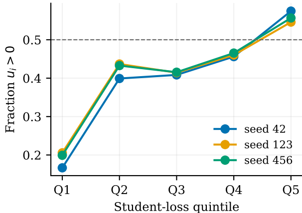
T_{a00} positive-utility fraction
