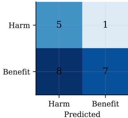
First-order
