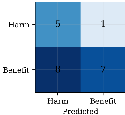
Second-order
