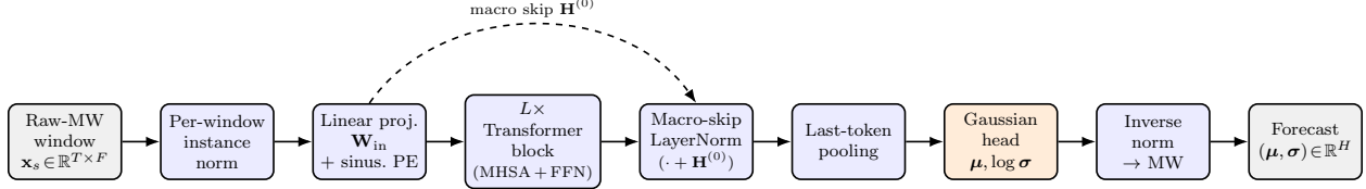
Figure 1: REnFormer architecture. A shared encoder processes each site’s lookback window independently. Each raw-MW window is renormalised by its own statistics, projected and position-encoded, passed through L post-LayerNorm Transformer blocks, and re-combined with the projected input via a macro skip connection (dashed). The last token is pooled and projected to Gaussian parameters for the forecast horizon, then de-normalised back to MW. Total: 536 k parameters.
