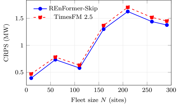
Figure 2: Probabilistic quality (CRPS, lower is better) versus fleet size. REnFormer-Skip (solid) sits below TimesFM 2.5 zero-shot (dashed) at every fleet size; the metric level tracks the mix of plant capacities added as N grows, not a monotone trend.
