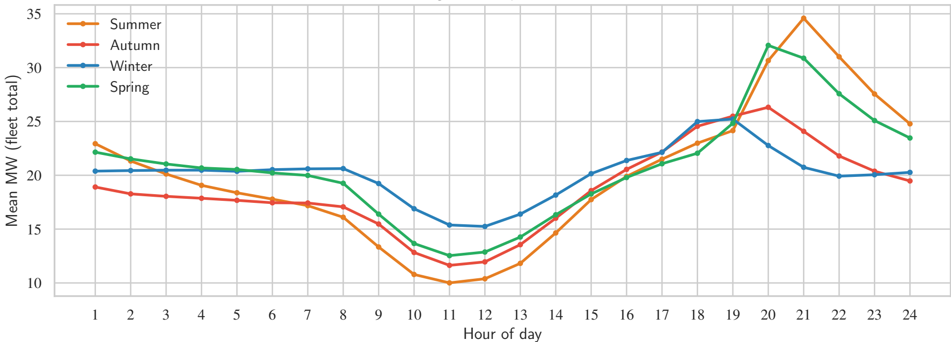
Diurnal generation profile — Eólicas
