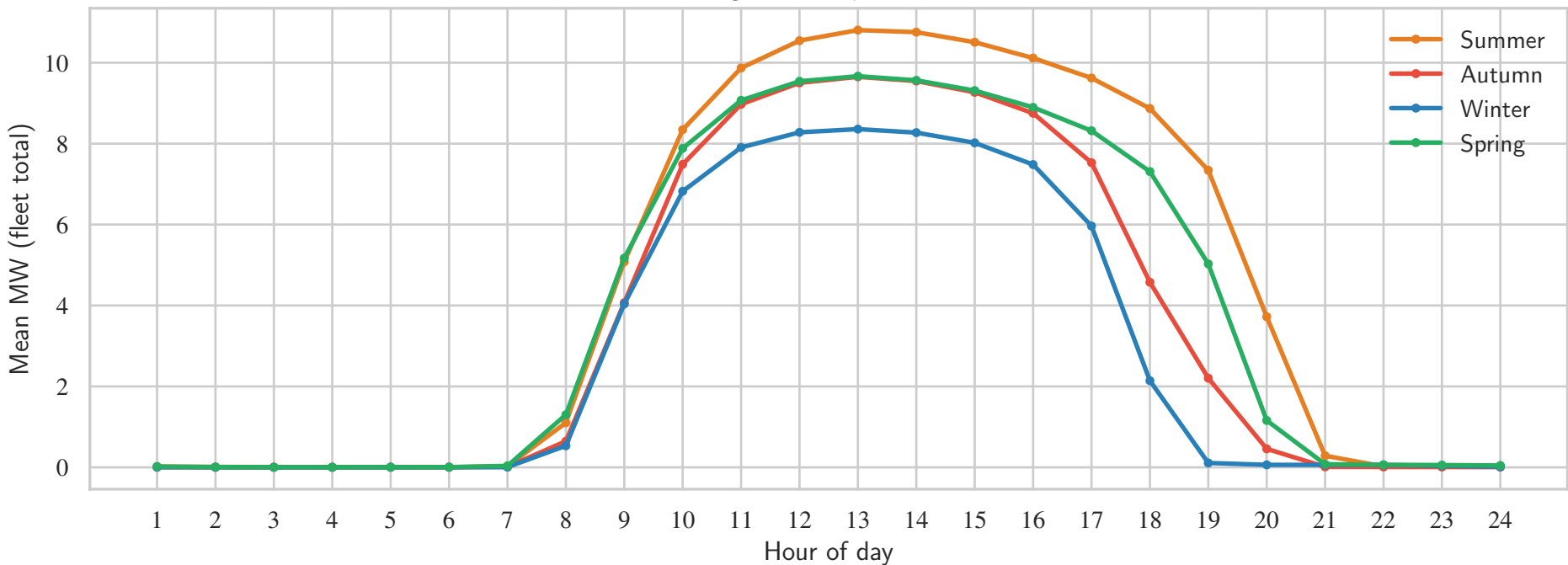
Diurnal generation profile — Solar
