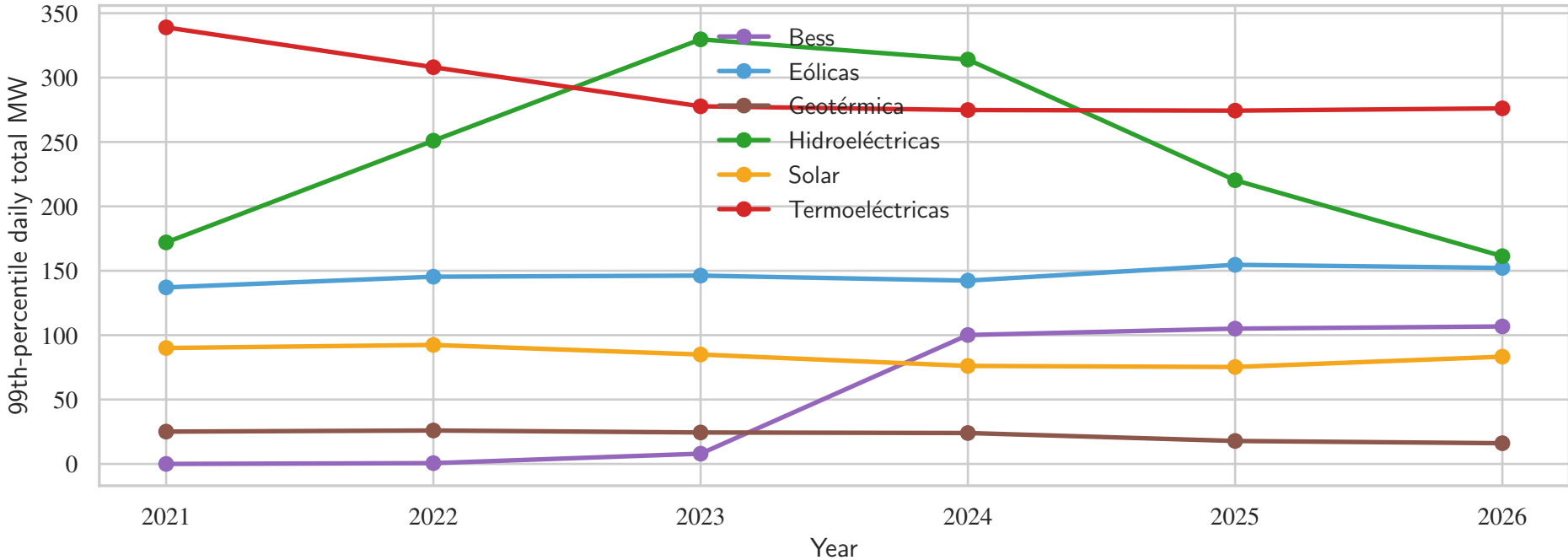
Fleet peak generation proxy (P99) by year
