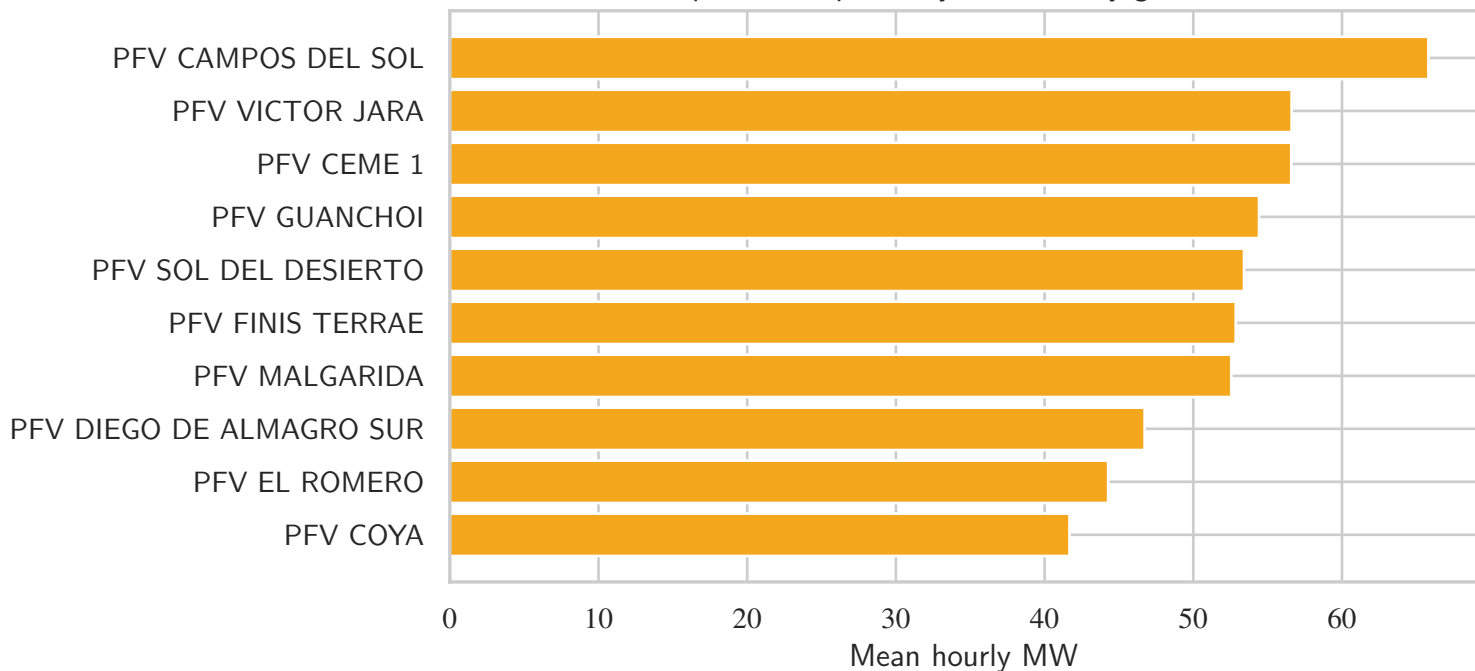
Top 10 Solar plants by mean hourly generation
