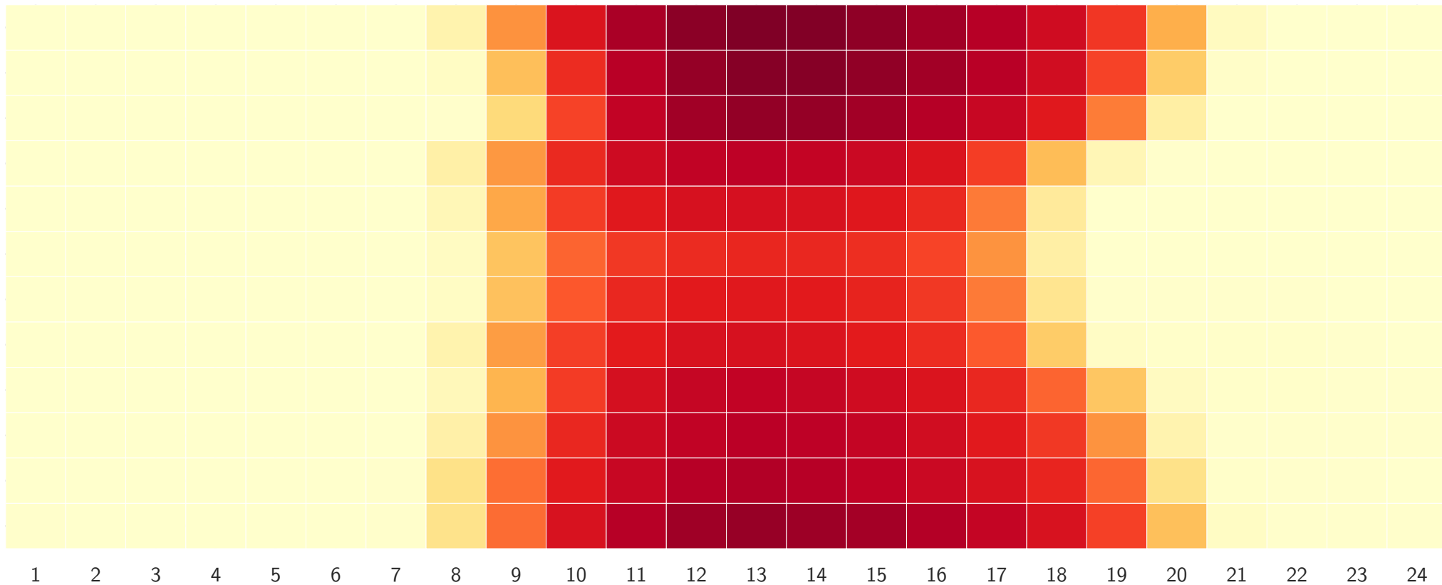
Solar fleet — mean hourly generation by month × hour
