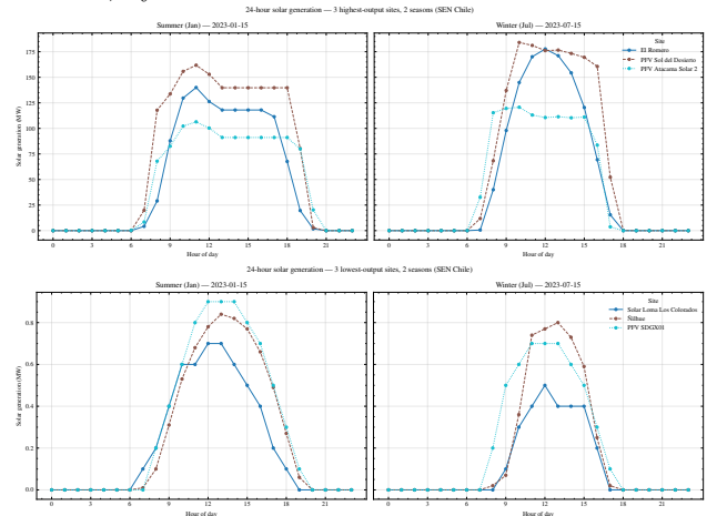
Figure 2: Highest and lowest generation sites in the test set, by season.
