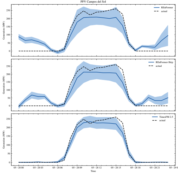
Figure 5: Last-window 24 h forecast for one site from three models.
