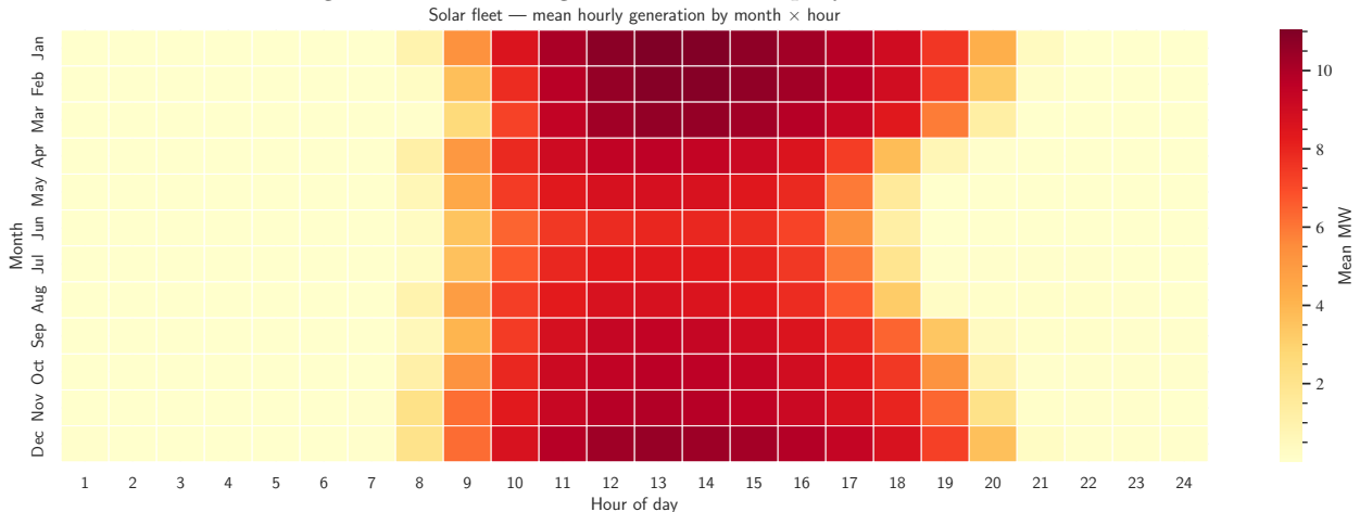
Figure 3: Solar fleet generation heatmap by month and hour.
