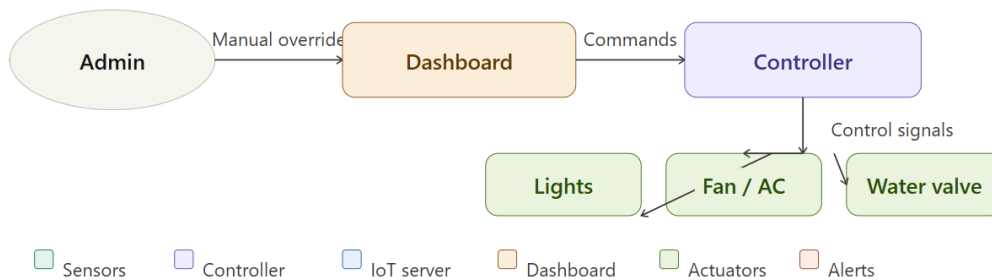
Figure 5: Control flow
