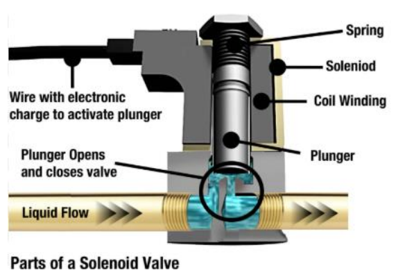
Figure 12: Solenoid valve components
