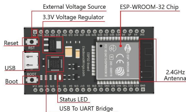
Figure 13: ESP32 processing unit
