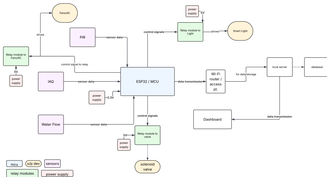
Figure 14: System integration diagram
