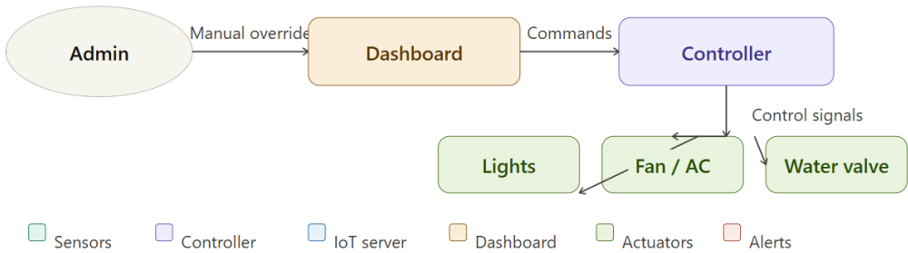
Figure 5: Control flow
