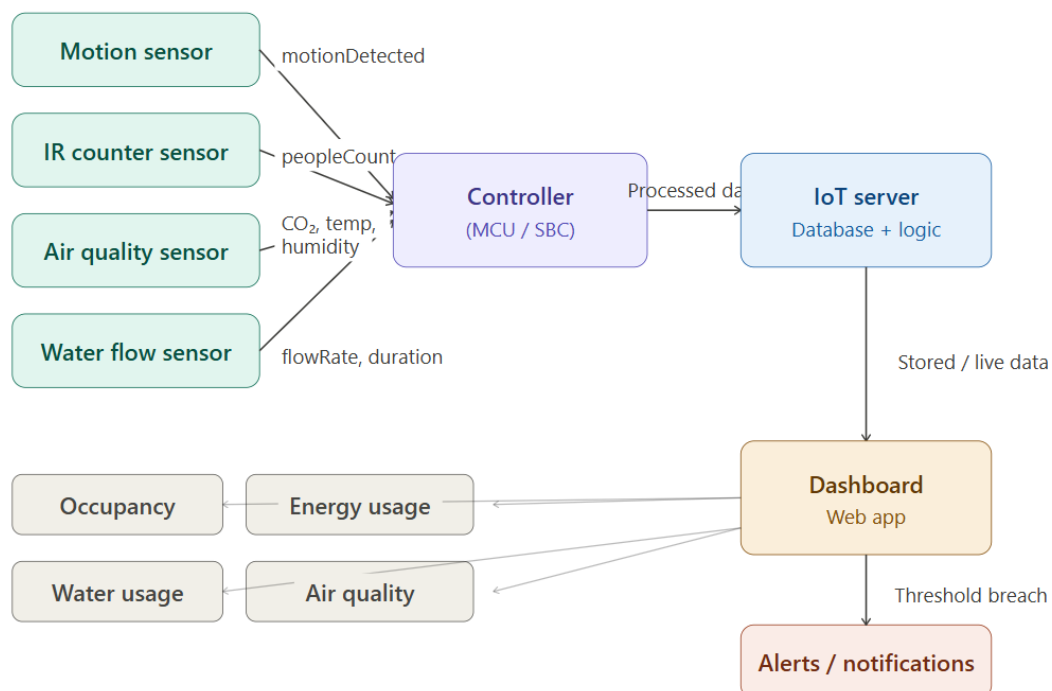
Figure 3: Main data flow
