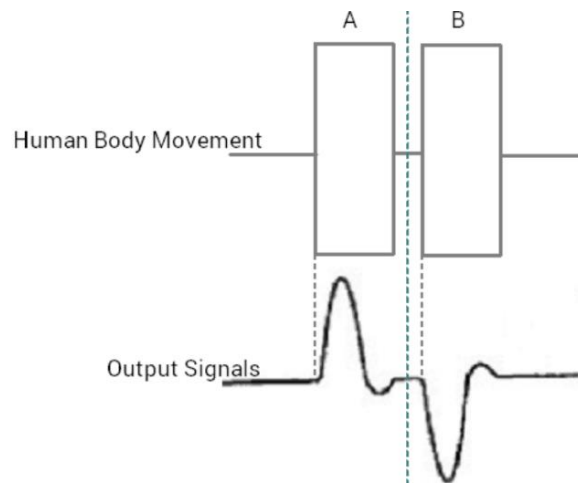
Figure 12: Motion detection behavior
