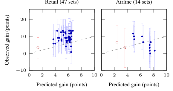
Figure 2: Each distinct deployed patch set’s gain over the unpatched agent as predicted from its bank replays (net of spurious recovery) against its observed held-out gain, with 90% intervals. Filled: sets containing the step-limit patch; open: sets without it. Dashed: y = x . Correlations are 0.23 (retail) and -0.49 (airline).
