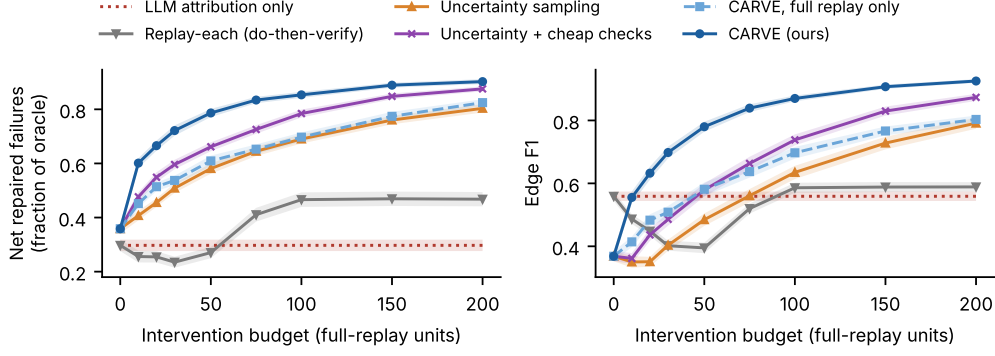
Figure 4: Net repaired failure mass (left) and edge F1 (right) against intervention budget, 50 worlds, shaded \pm 1 s.e.
