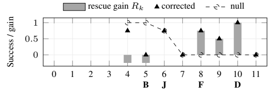
Figure 1: Rescue profile of one retail failure (null replays only where some sample corrected). The agent listed two 4K waterproof cameras but proposed the silver one, which the user accepted; the task names no colour, and the grading expects the cheaper black one. At step 6 (J: all-at-once judges) corrected and null replays both succeeded three times in four. At steps 8–10 (F: first write; D: best rescue step) the oracle rescued by swapping in the black camera, overriding the user’s confirmed choice, a kind both auditors rejected. B: binary search.
