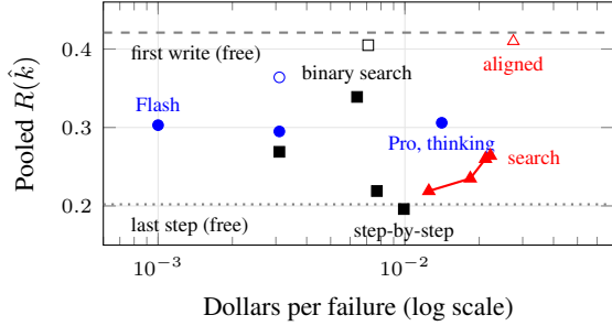
Figure 3: Rescue score against cost. Circles: all-at-once judges; squares: other LLM methods; triangles: counterfactual search at budgets 8, 16, 24 and 40. The free first-write rule lies above every registered method. Open markers (post hoc): the all-at-once judge and binary search asked for the largest gain, and aligned search.
