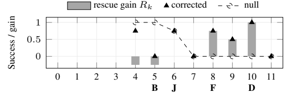
Figure 1: Rescue profile of one retail failure over agent steps (null replays only where some sample corrected). The user, offered two 4K waterproof cameras, chose the silver one; the grading expected the black one. At step 6 (J: all-at-once judges) corrected and null replays both succeeded three times in four, a recovery without correction. At steps 8–10 (F: first write; D: best rescue step) the oracle rescued by swapping in the black camera, overriding the user’s confirmed choice, a kind of correction both auditors rejected (§5). B: binary search.
