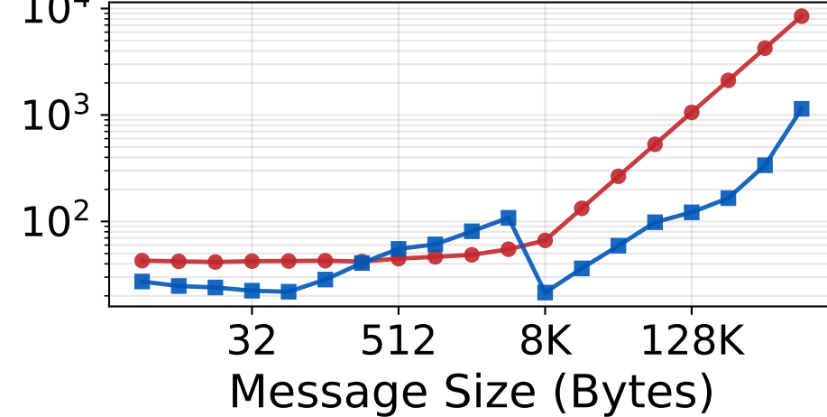
Allreduce
