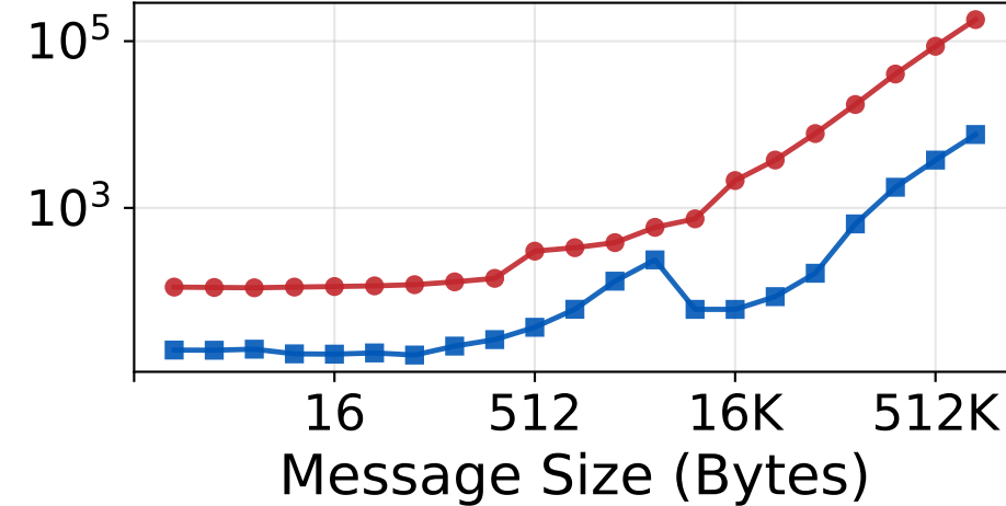
Alltoall
