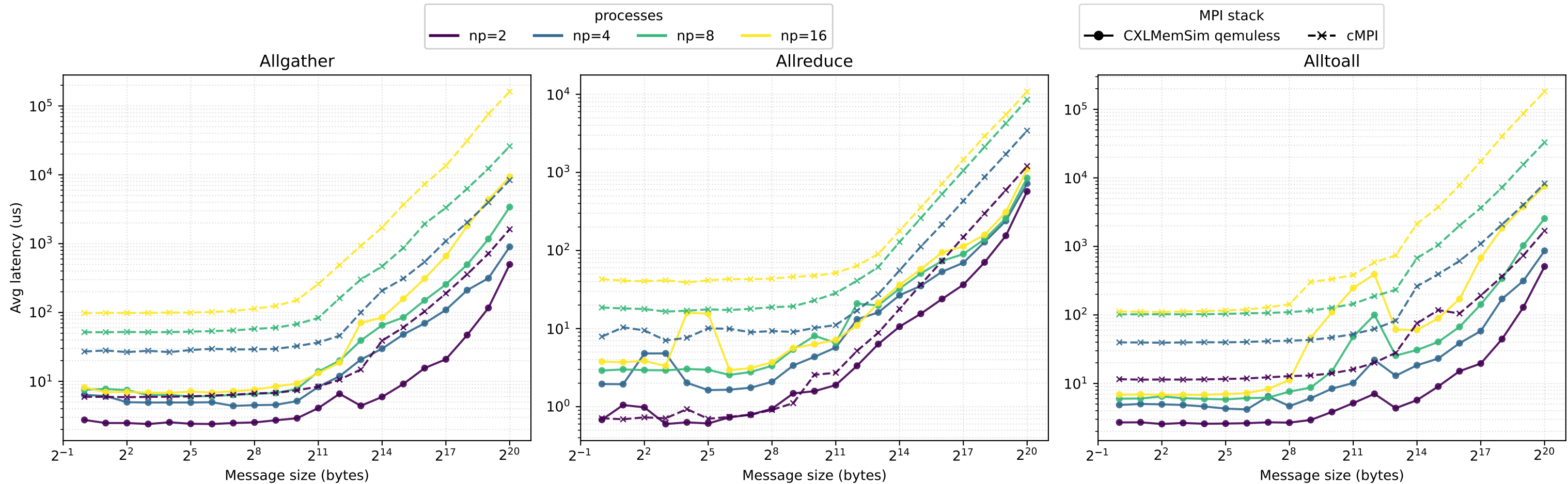
OSU collective latency: CXLMemSim qemiless vs cMPI (single node, nocc)
