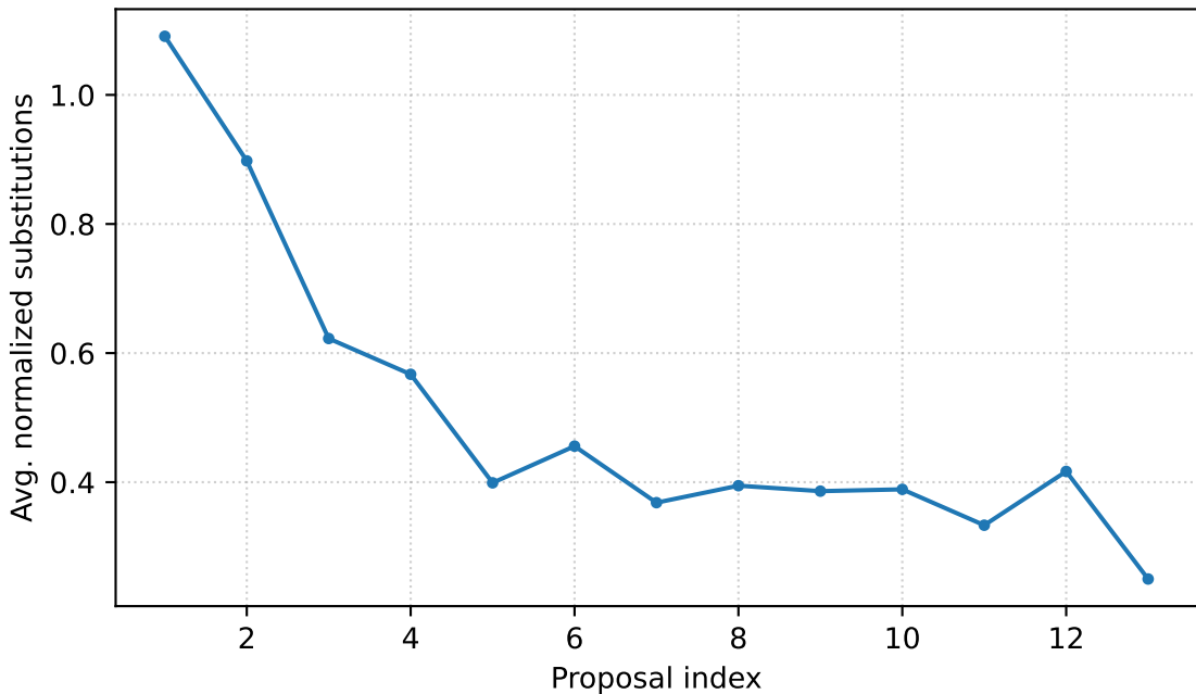
Avg. Normalized substitutions over proposal idx gpt-5-2025-08-07-no-reasoning-t1.0 - opposite goals experiments
