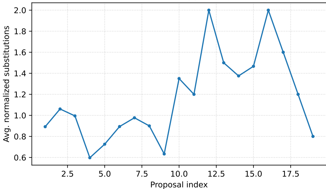
Avg. Normalized substitutions over proposal idx llama-3.3-70b-instruct-t1.0 - opposite goals experiments
