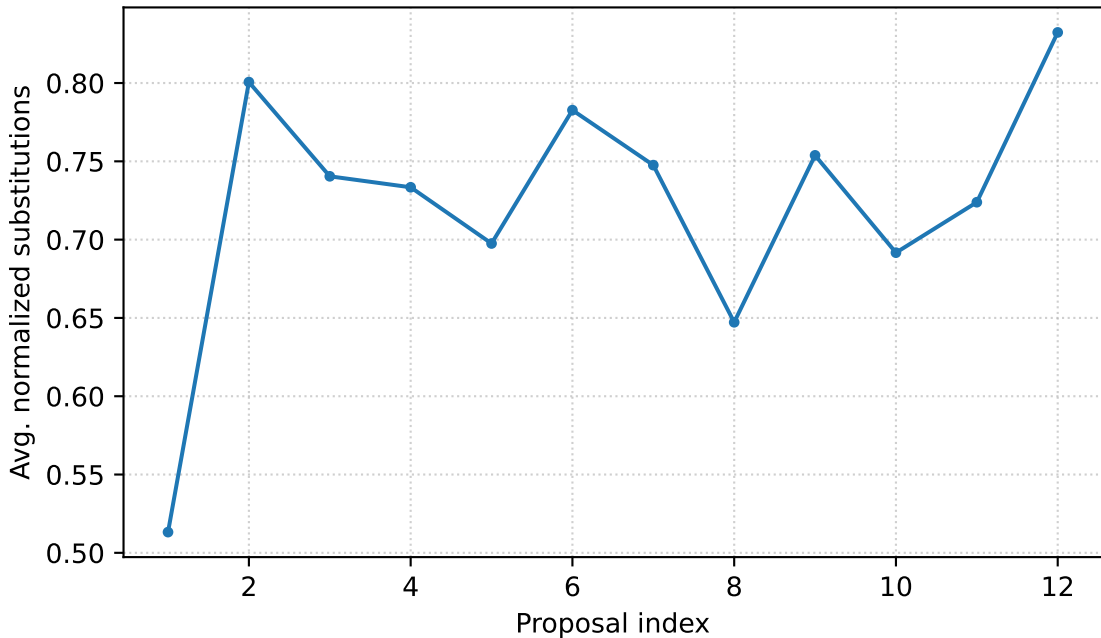
Substitutions over proposals in temporal order GPT-OSS 120B
