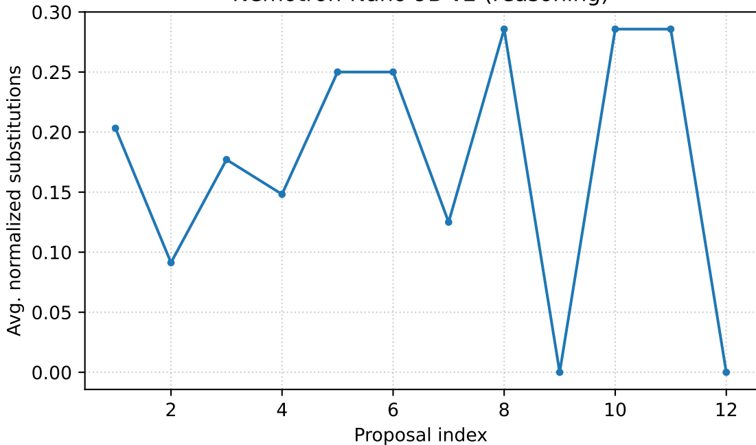
Substitutions over proposals in temporal order Nemotron-Nano 9B v2 (reasoning)
