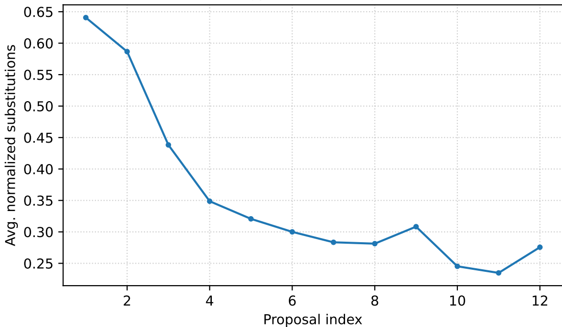
Substitutions over proposals in temporal order gpt-5-reasoning
