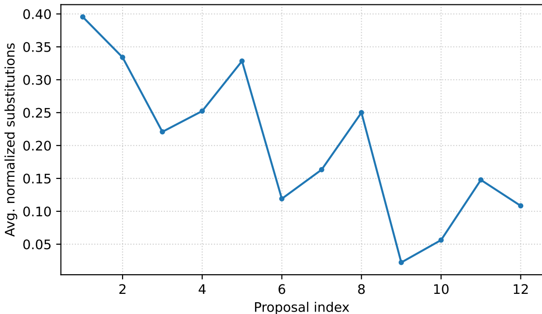
Substitutions over proposals in temporal order nemotron-nano-9b-v2-noreasoning
