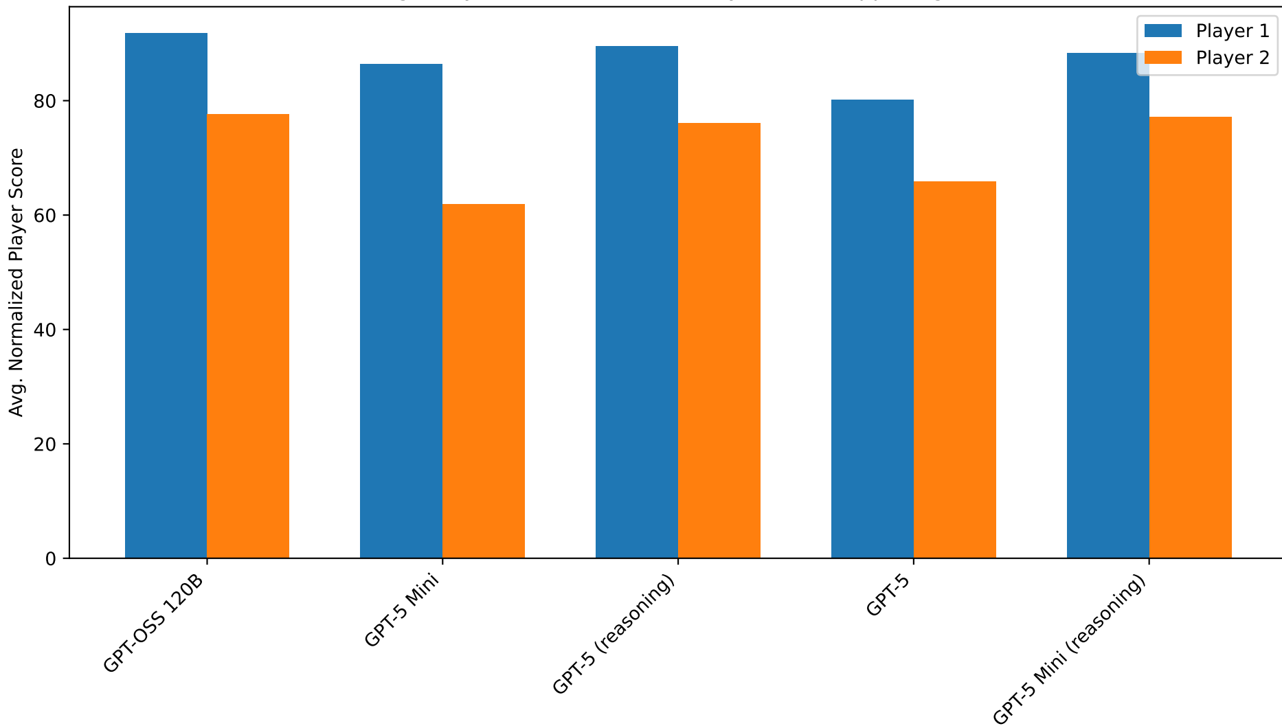
Average Player Scores for GPT-family Models (Opposing Goals)
