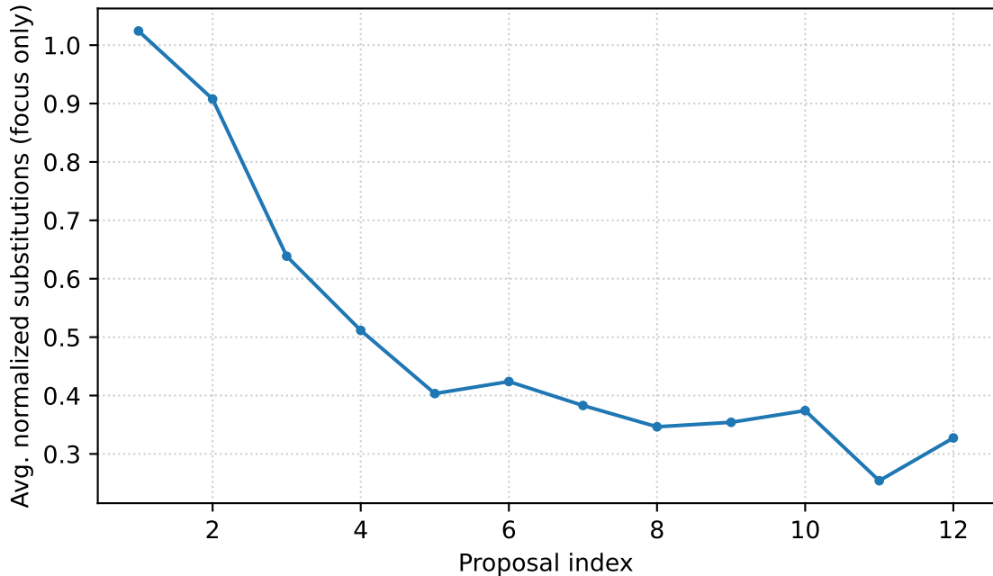
Substitutions over proposals (focus experiments) GPT-5
