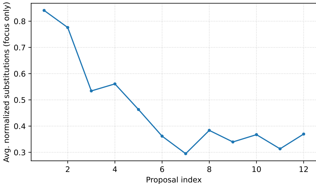
Substitutions over proposals (focus experiments) GPT-5 Mini
