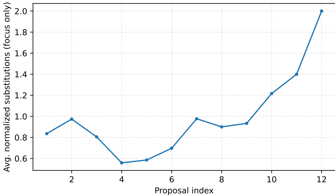
Substitutions over proposals (focus experiments) LLaMA-3.3-70B Instruct
